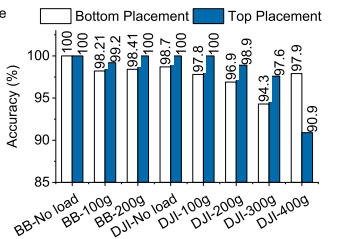
Figure 23: Estimation accuracy at different placement
