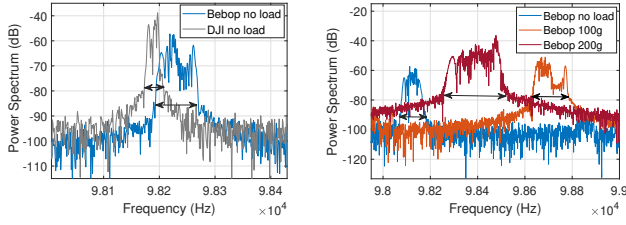
Figure 11: (Left) DJI and Bebop vibration profile captured by RF signal, (Right) Bebop vibration profile when carrying external load captured by RF signal
