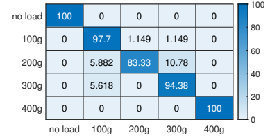
Figure 19: Mavic 2 load estimation accuracy
